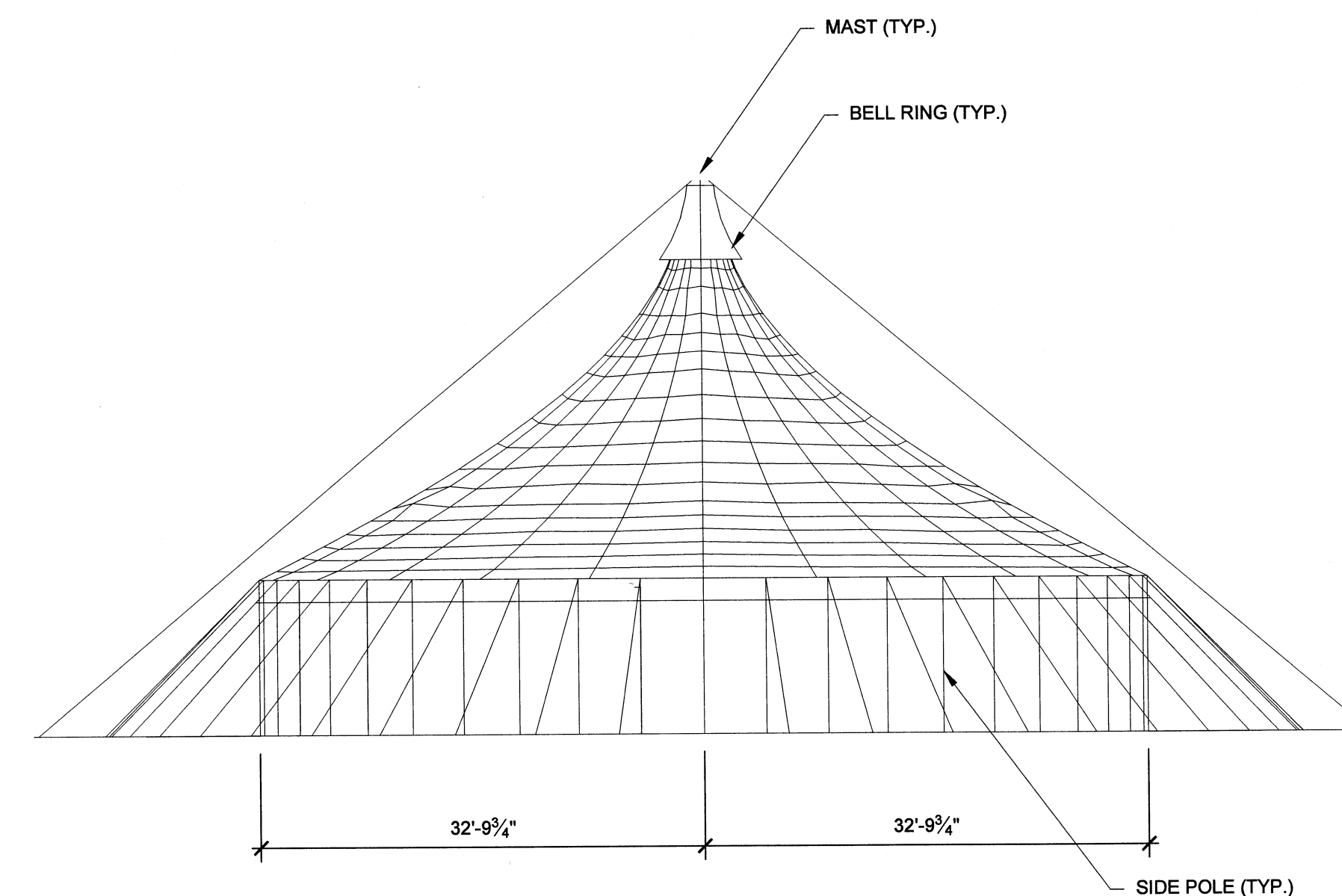
3 TENT END VIEW SCALE: 3/32" = 1'-0"
