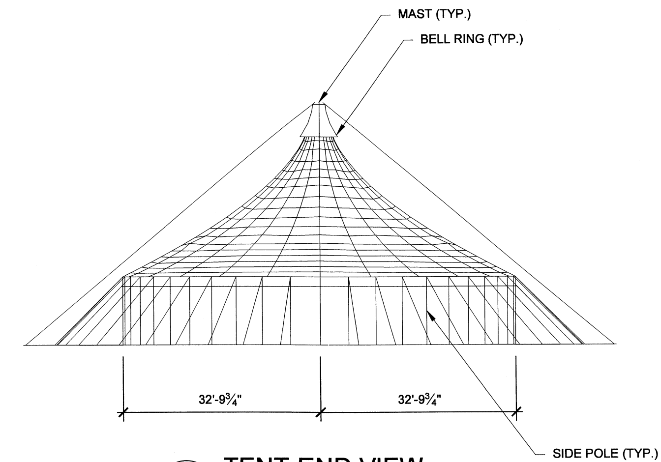
3 TENT END VIEW SCALE: 3/32" = 1'-0"
