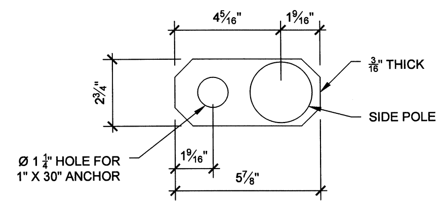
7 DINING TENT SIDE POLE BASE PLATE SCALE: 3" = 1'-0"
