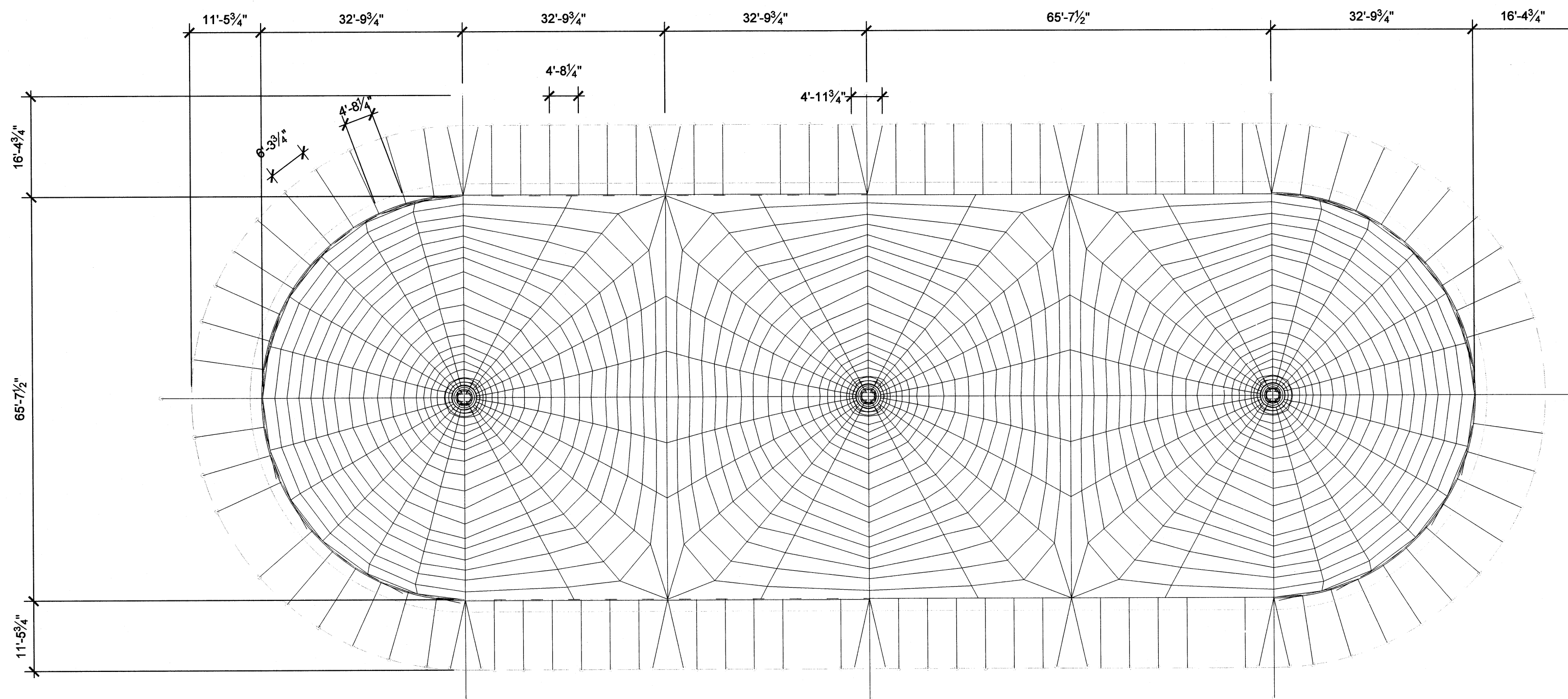
1 TENT PLAN SCALE: 3/32" = 1'-0"
