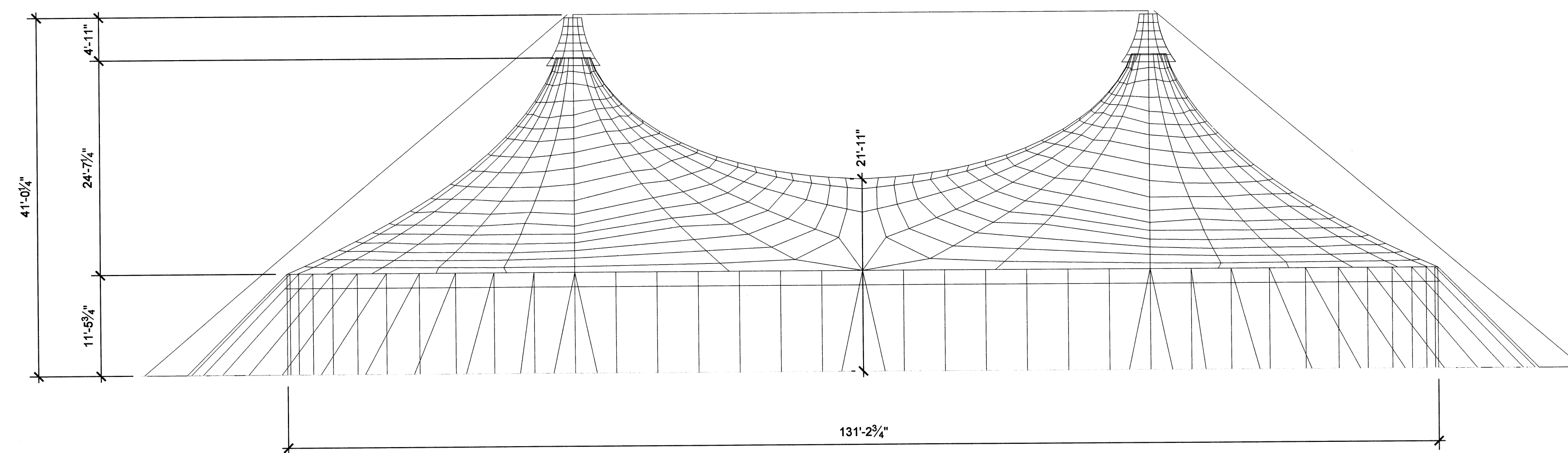
2 TENT SIDE VIEW SCALE: 3/32" = 1'-0"
