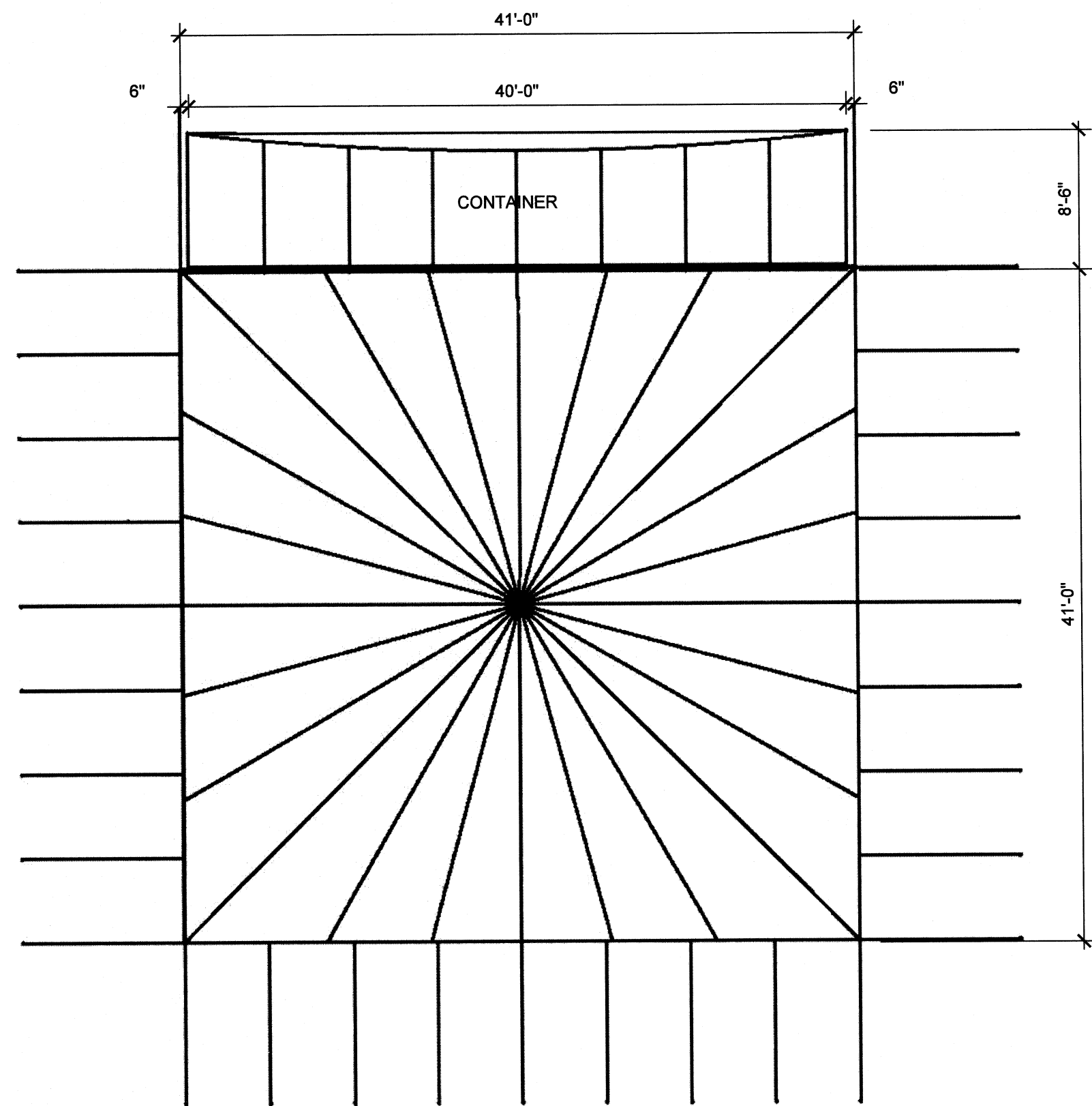
1 DINING TENT PLAN SCALE: 1/8" = 1'-0"
