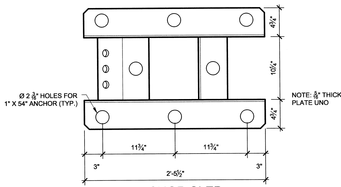
4 ANCHOR SLED SCALE: 1 1/2" = 1'-0"
