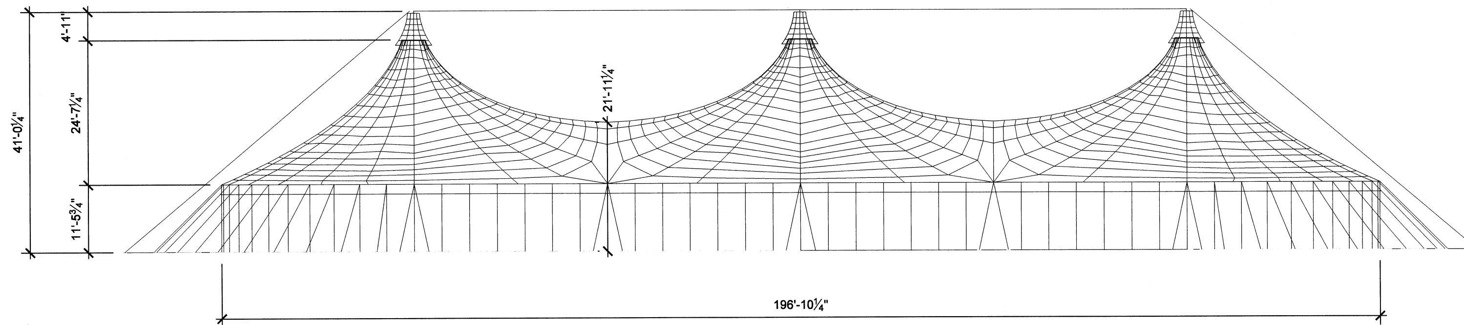
2 TENT SIDE VIEW SCALE: 3/32" = 1'-0"
