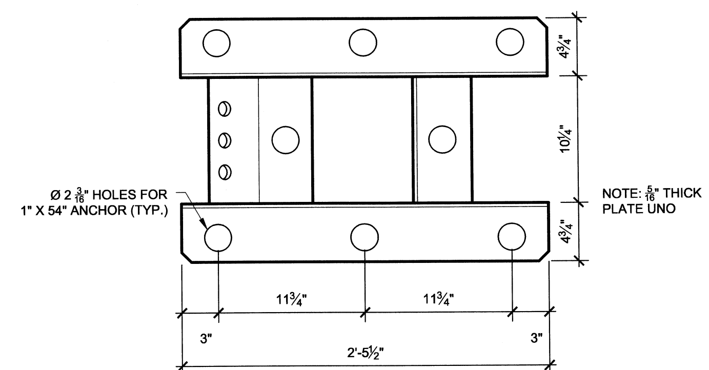
4 ANCHOR SLED SCALE: 1 1/2" = 1'-0"
