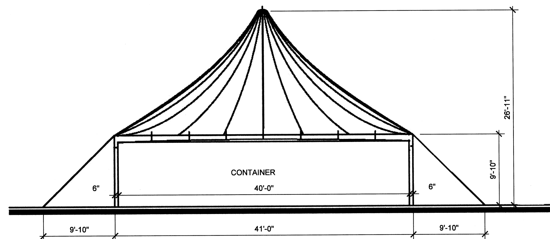
3 DINING TENT ELEVATION SCALE: 1/8" = 1'-0"
