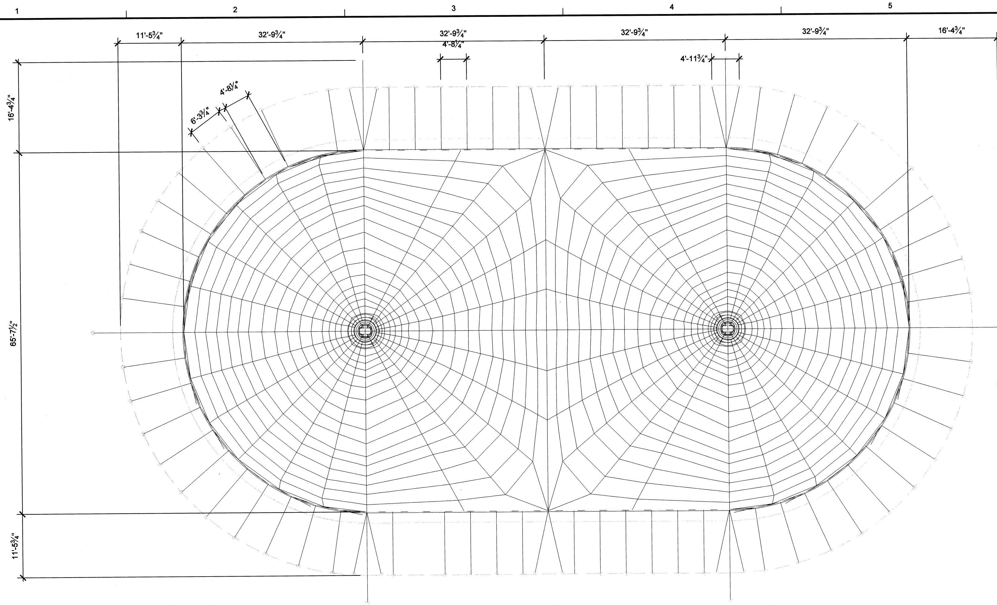
1 TENT PLAN SCALE: 3/32" = 1'-0"
