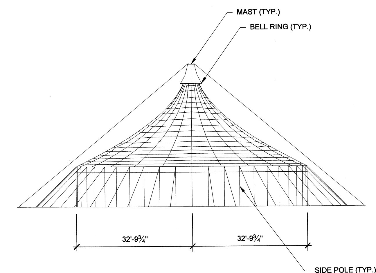
3 TENT END VIEW SCALE: 3/32" = 1'-0"
