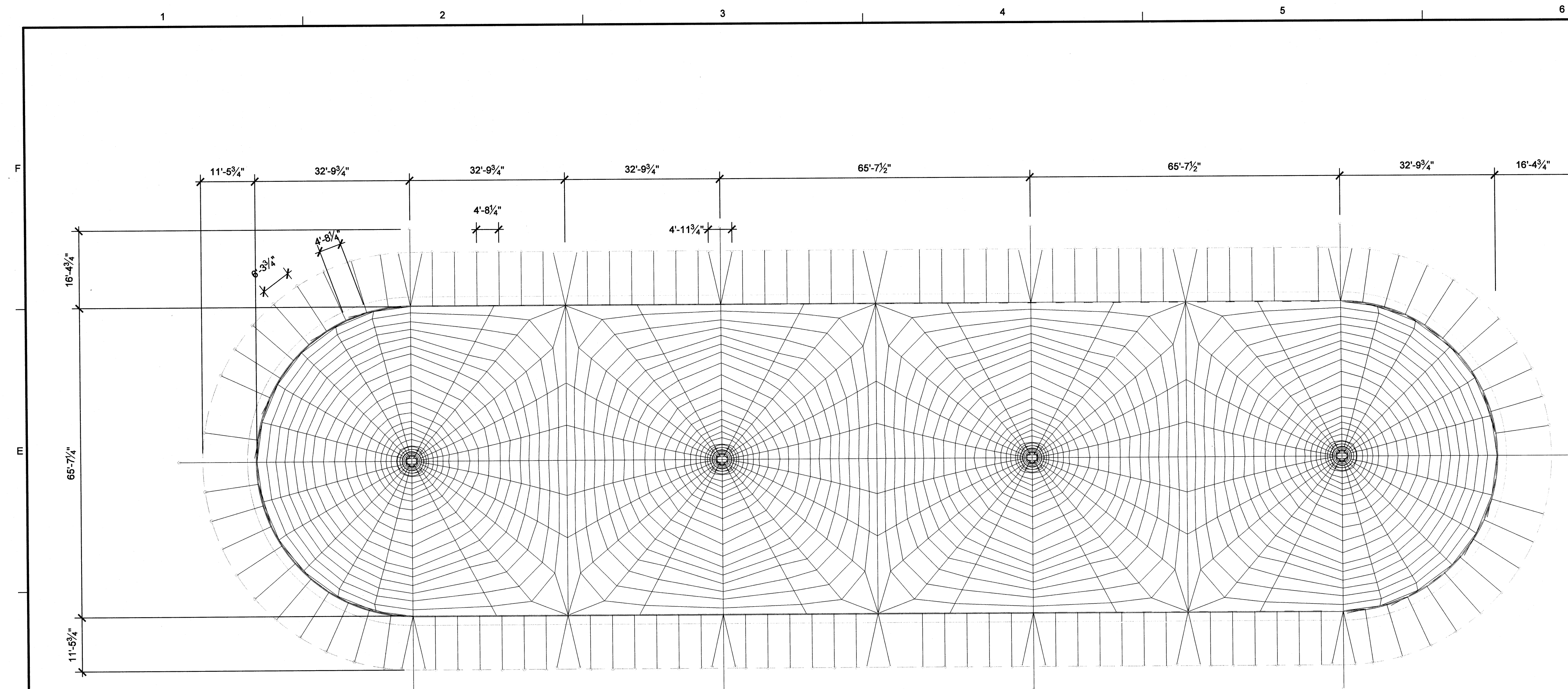
1 TENT PLAN SCALE: 3/32" = 1'-0"
