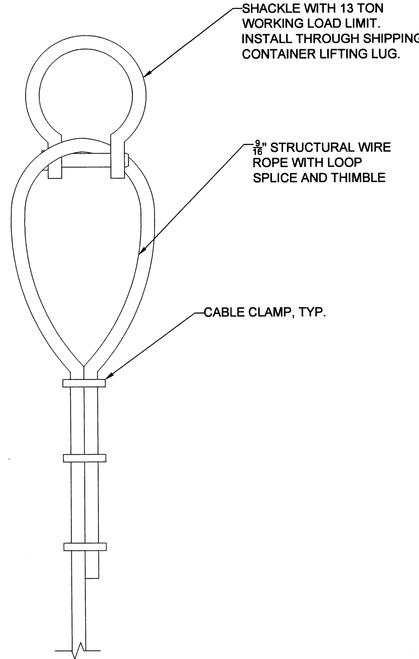
3 ATTACHMENT DETAIL SCALE: 3/8" = 1'-0"
