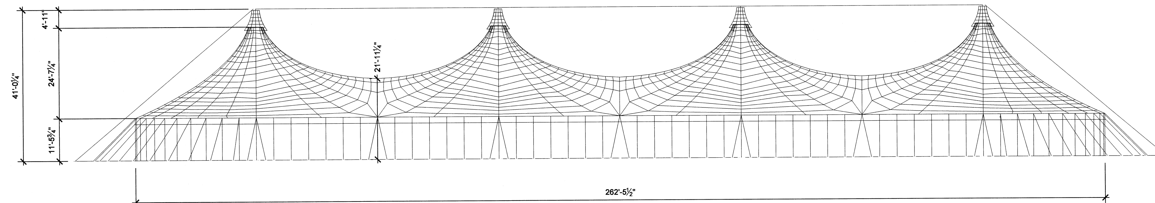
2 TENT SIDE VIEW SCALE: 3/32" = 1'-0"
