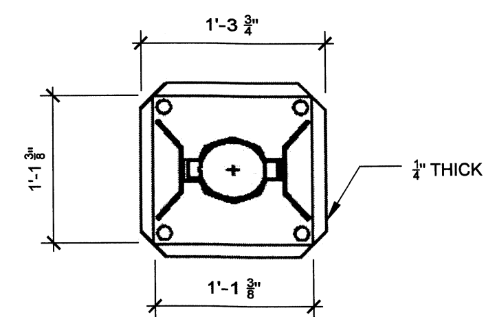
9 DINING TENT MAST BASE PLATE SCALE: 1" = 1'-0"
