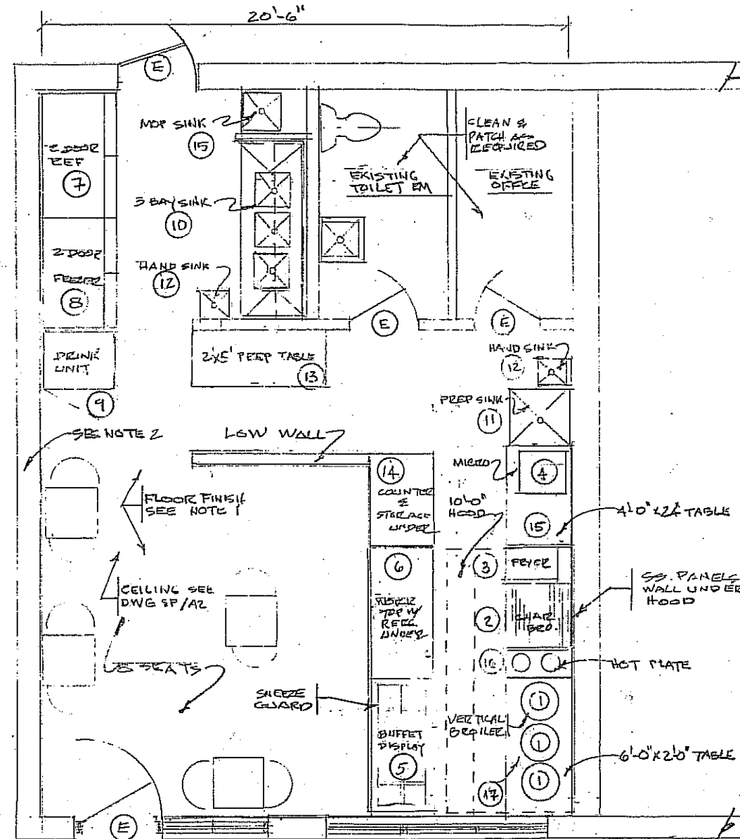
FLOOR PLAN 1/4" x 1/2" (574 SF)
