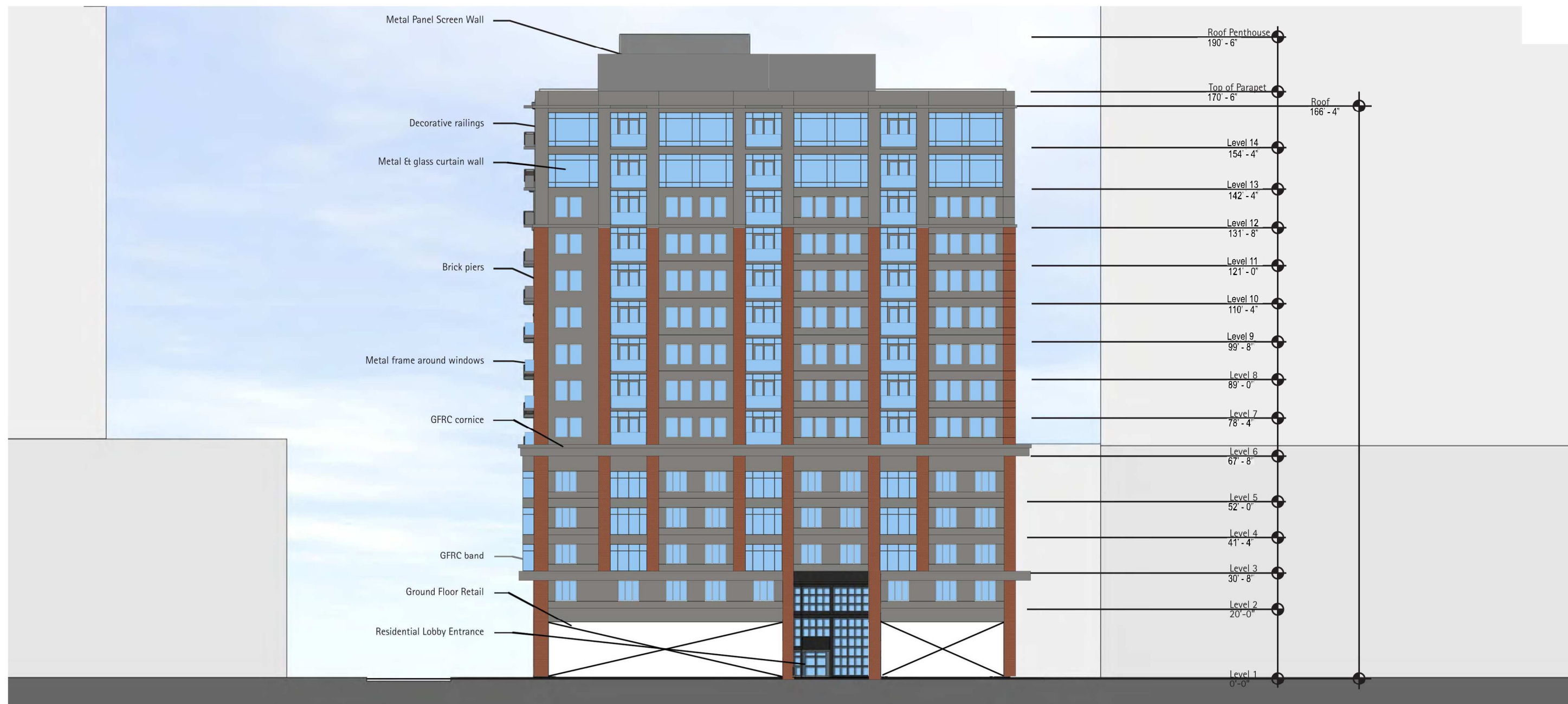
North Elevation: Canal St
