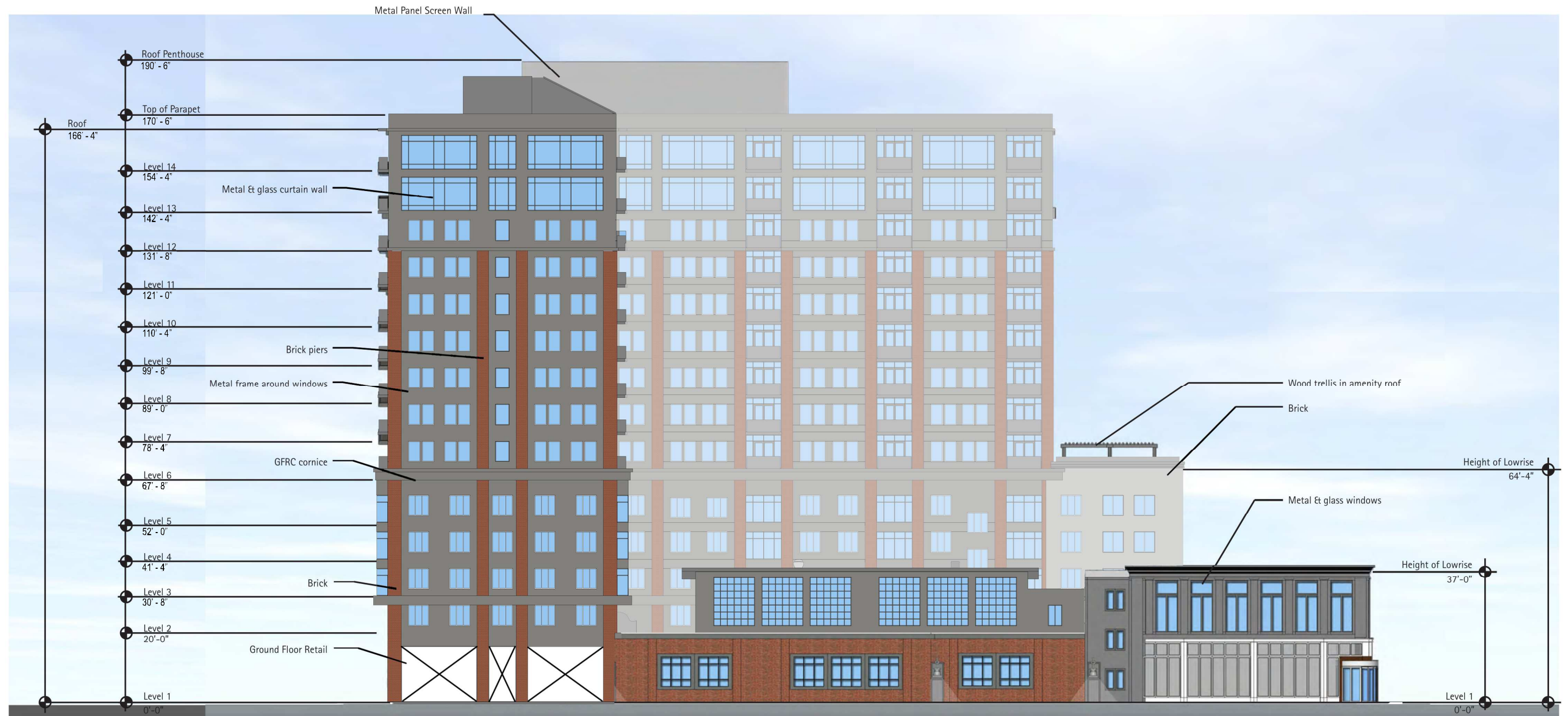
West Elevation: Alley
