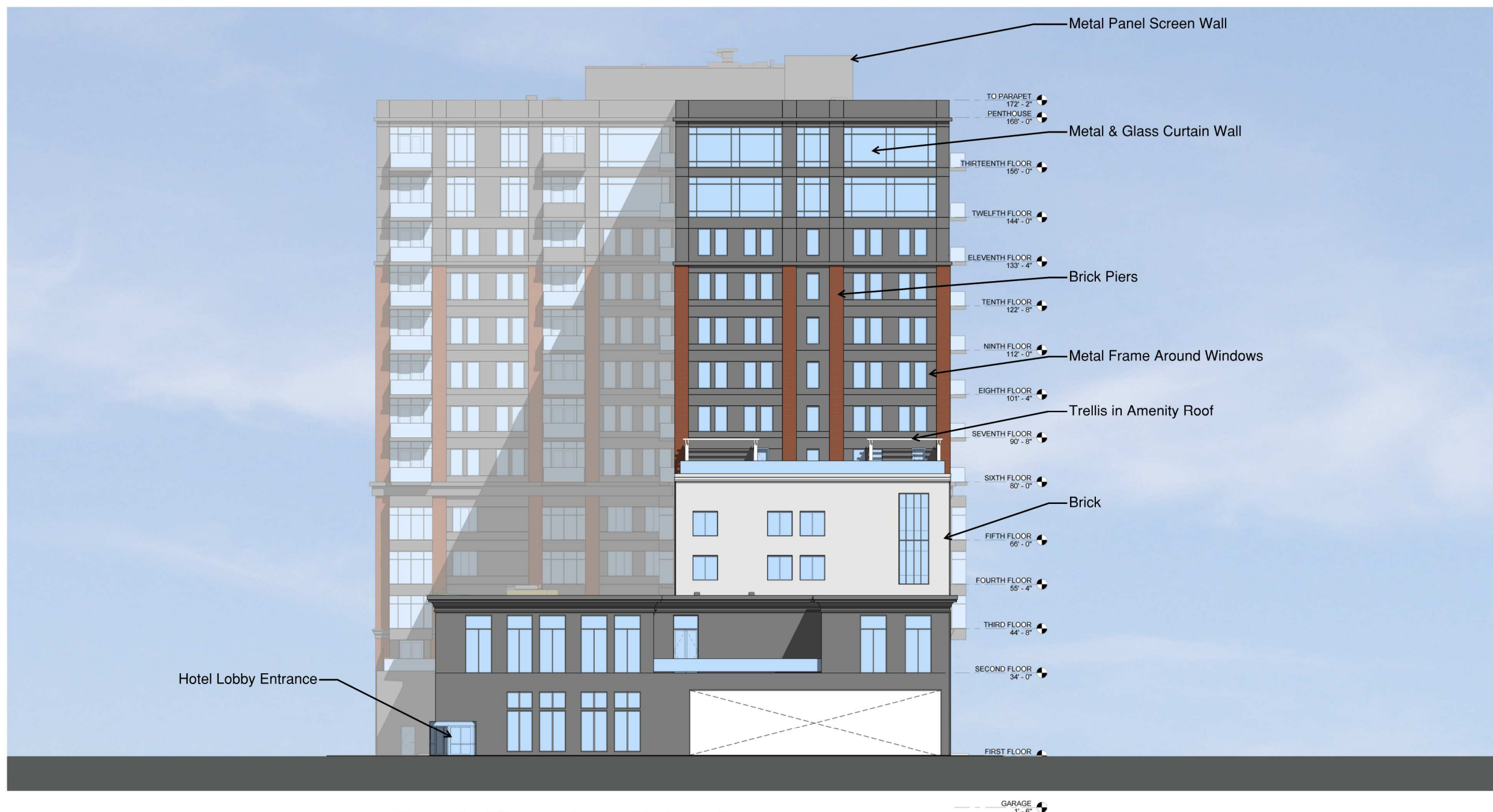
South Elevation: Foley Street
