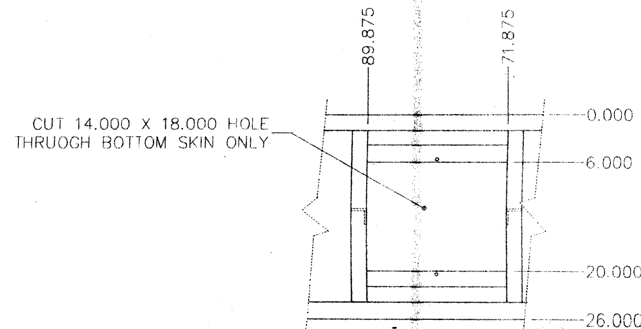
BOTTOM SOCKET DETAIL
