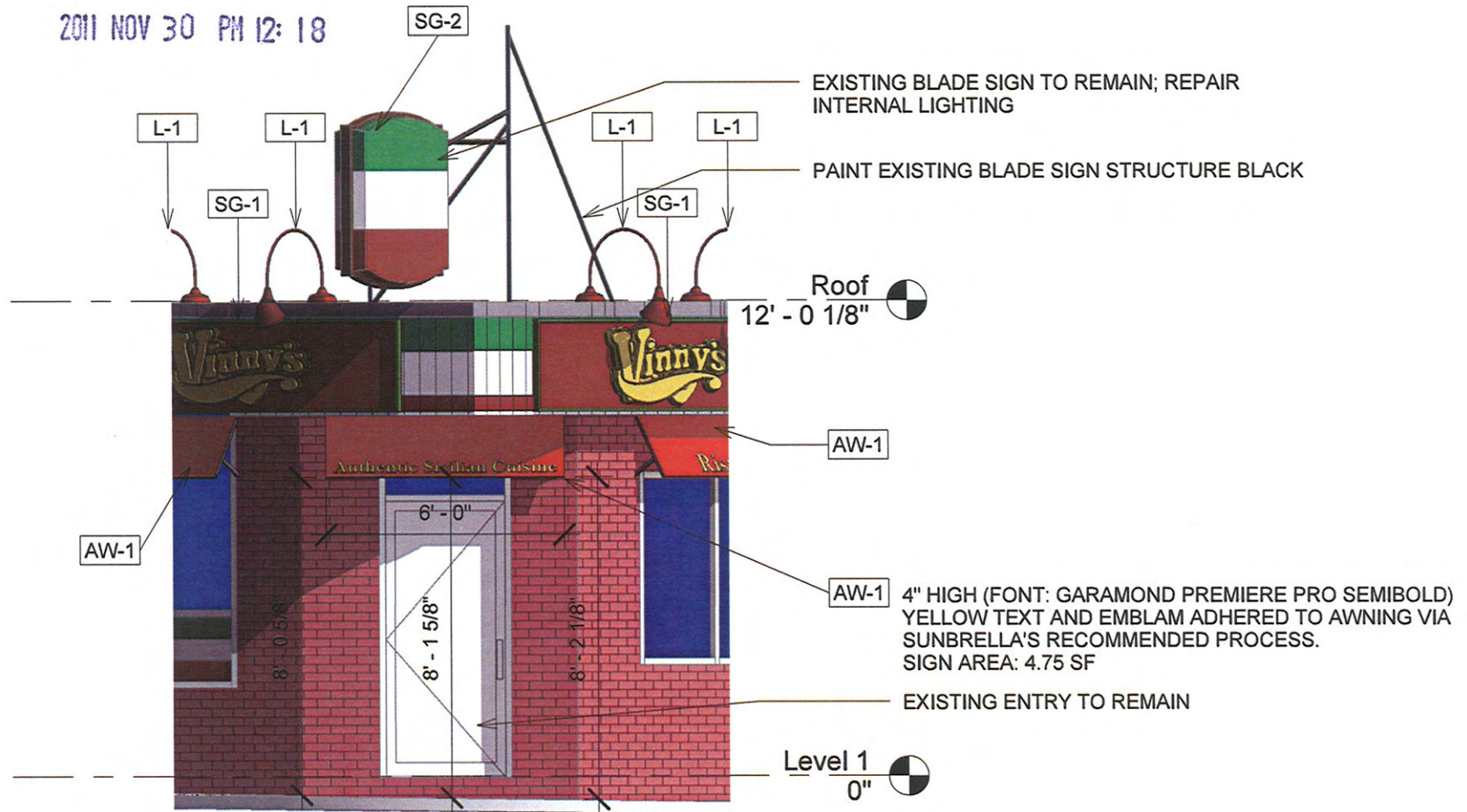
1 Entry Elevation 1/4" = 1'-0"
