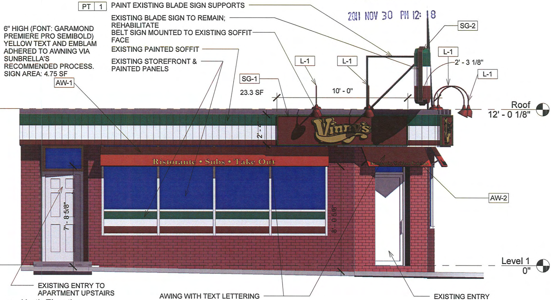
1 North Elevation 1/4" = 1'-0"
