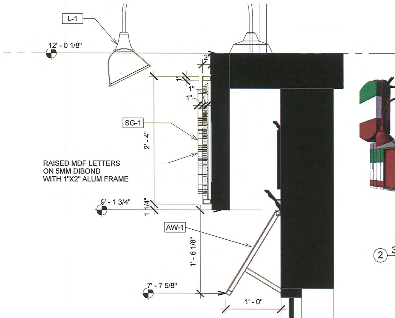
1 Sign Section 1" = 1'-0"
