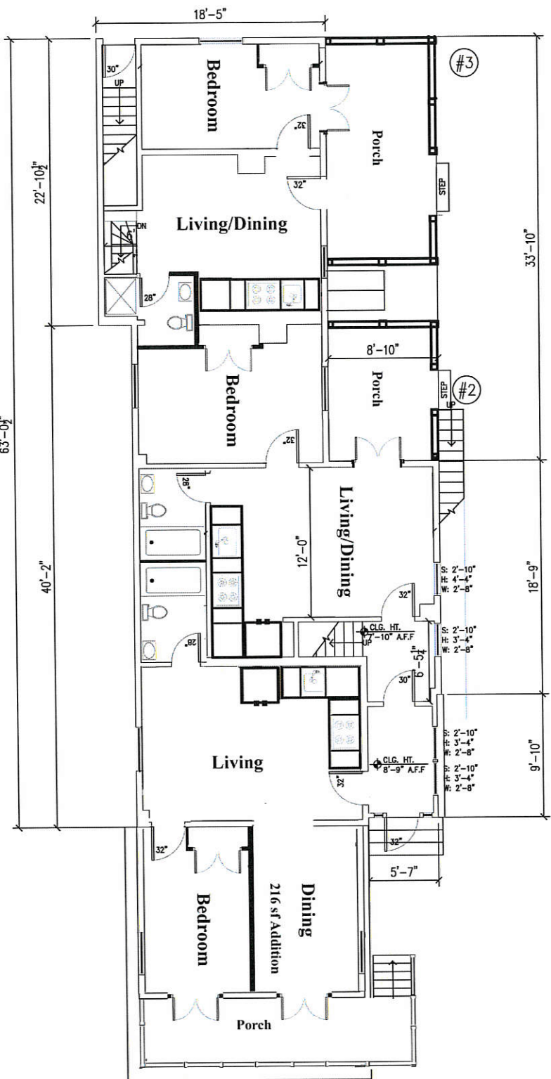
FIRST FLOOR PLAN 1,272 sf NFA TOTAL
