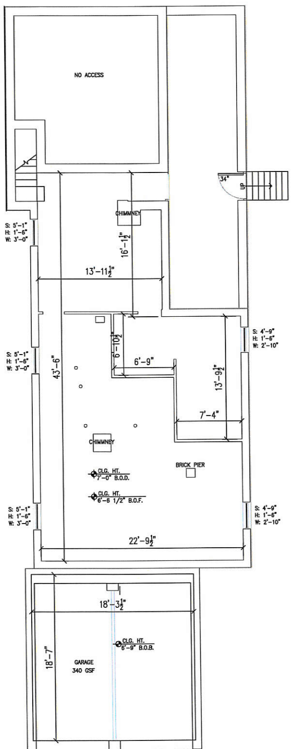
BASEMENT FLOOR PLAN 0 sf NFA TOTAL
