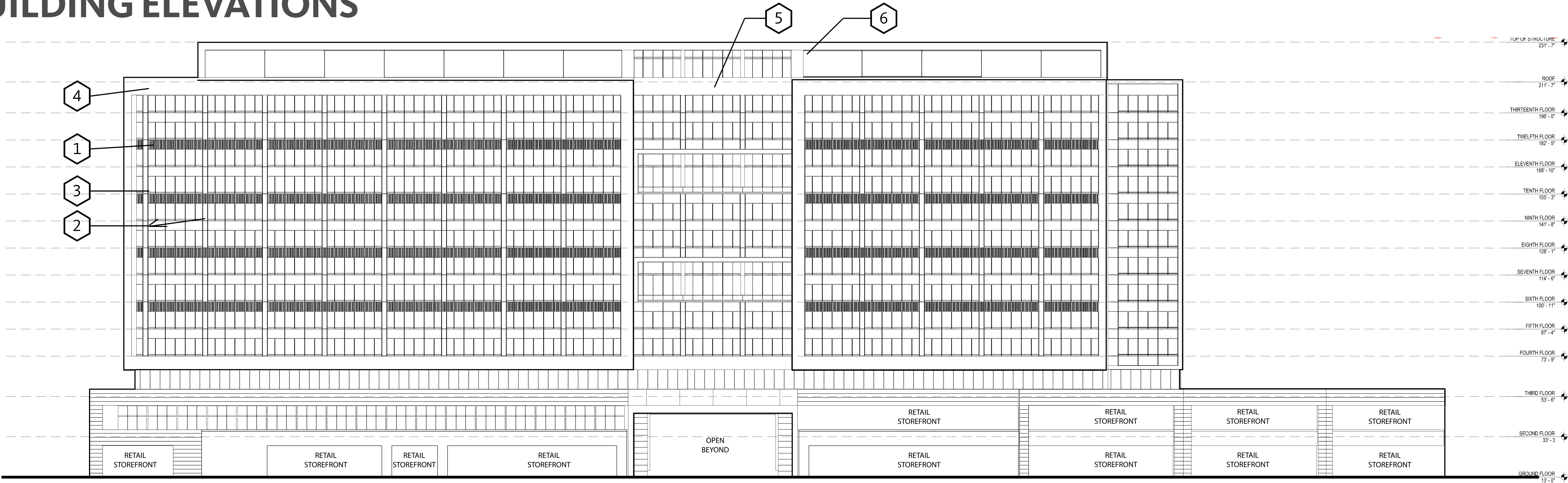
NORTH ELEVATION | 1"-16'-0"
