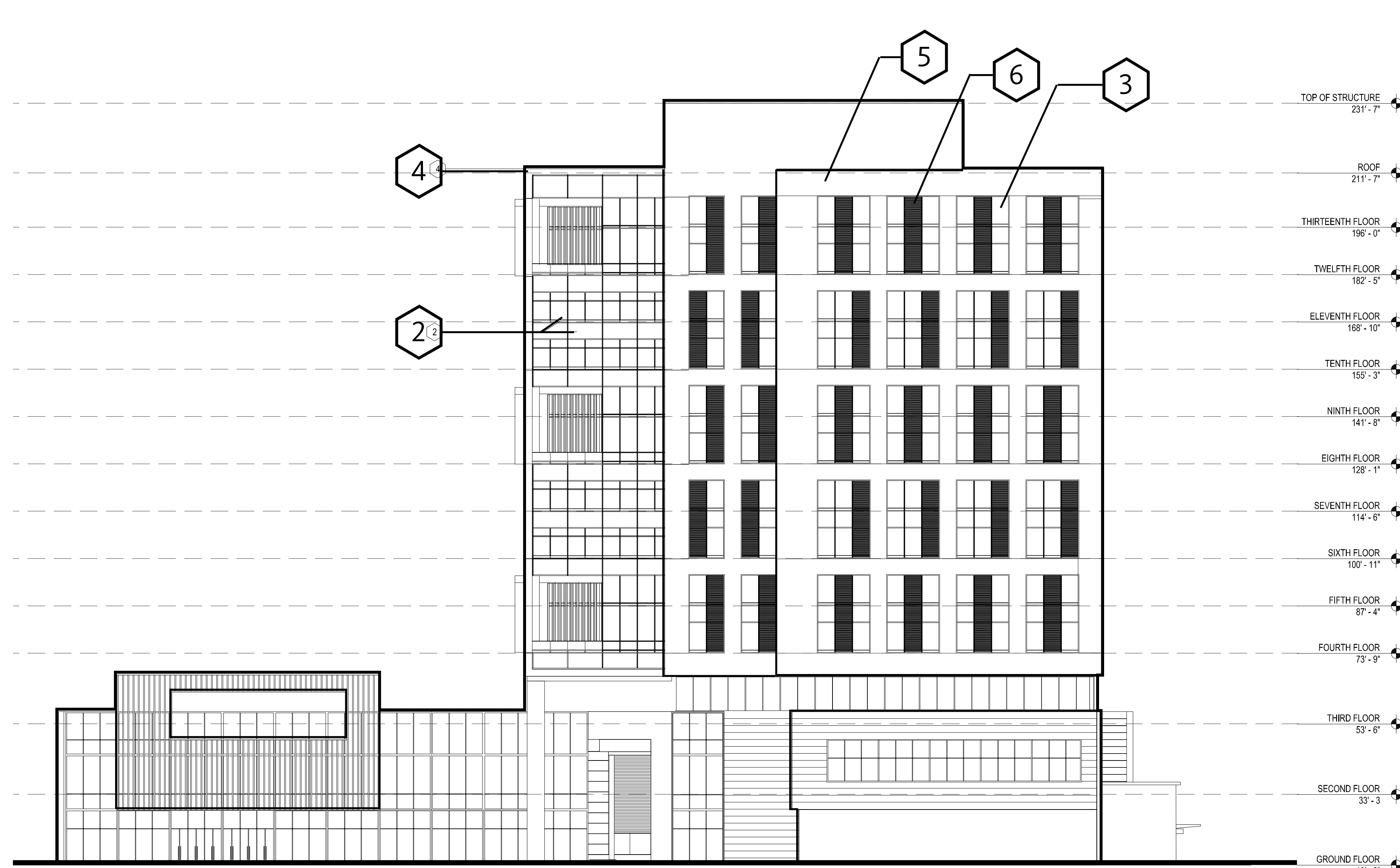
EAST ELEVATION | 1"-16'-0"
