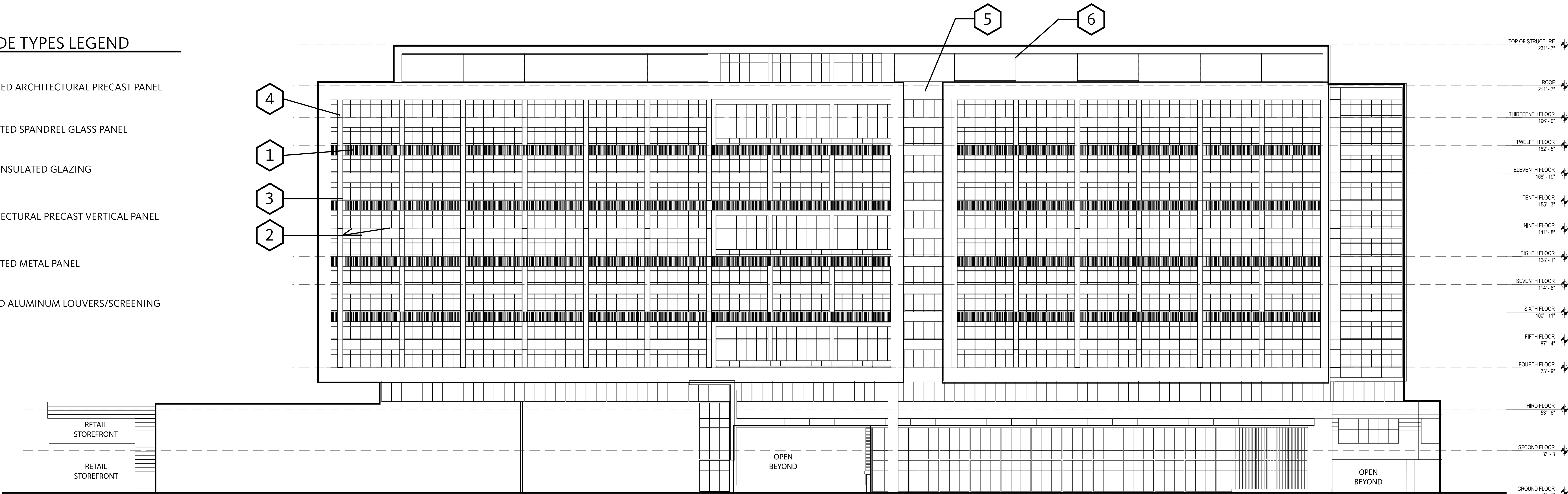
SOUTH ELEVATION | 1"-16'-0"
