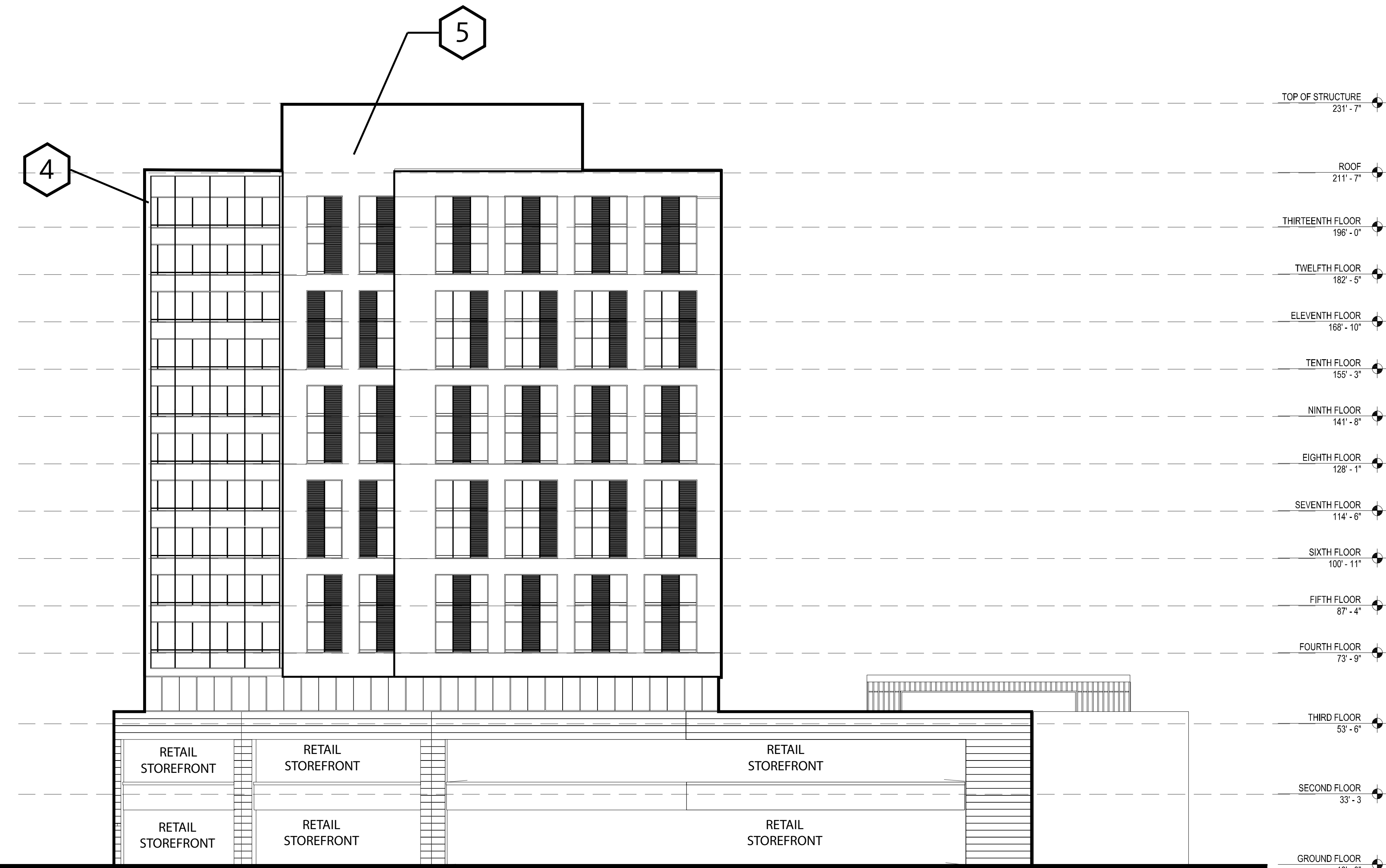
WEST ELEVATION | 1"-16'-0"
