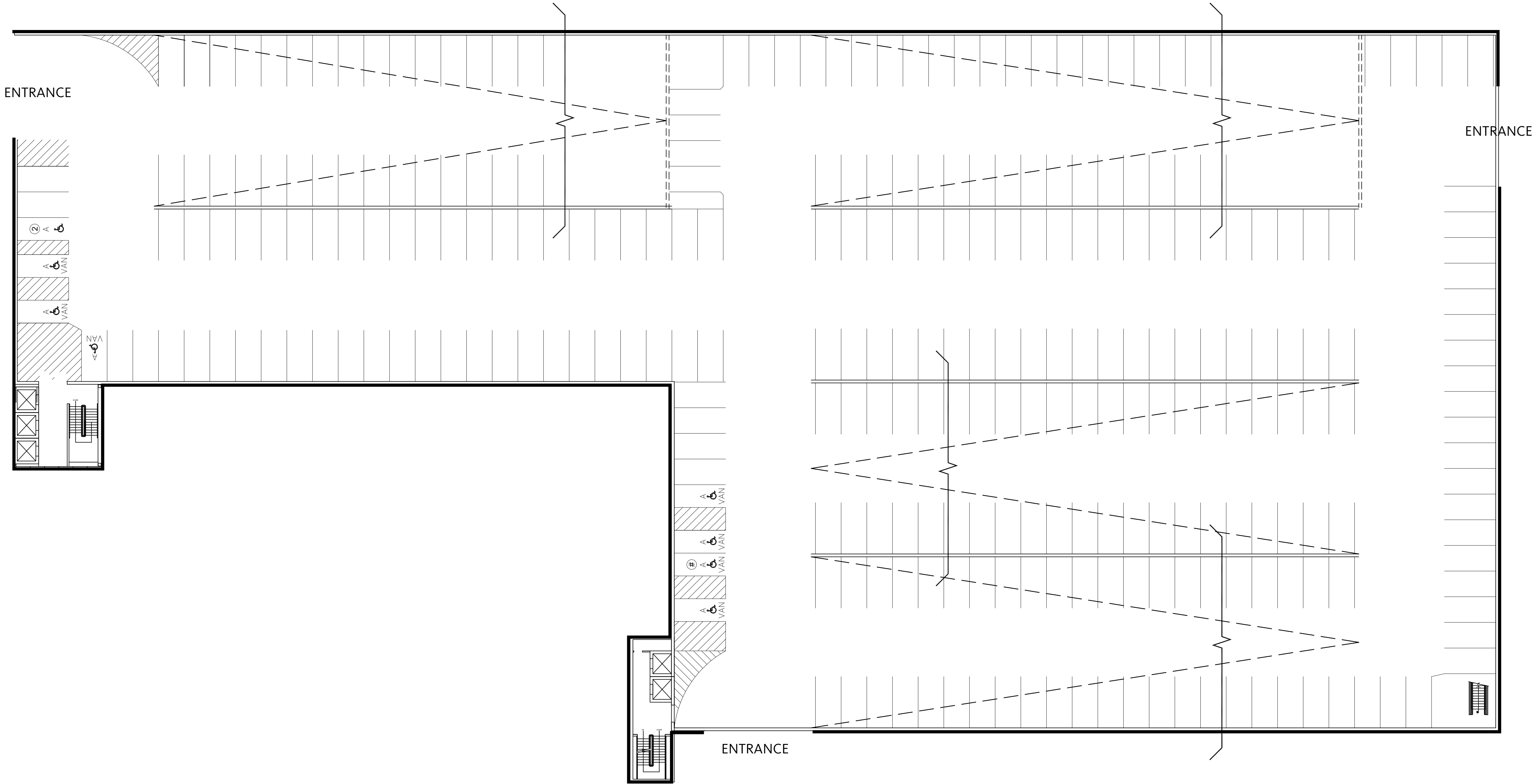
GROUND LEVEL PLAN | 1"-20'-0"
