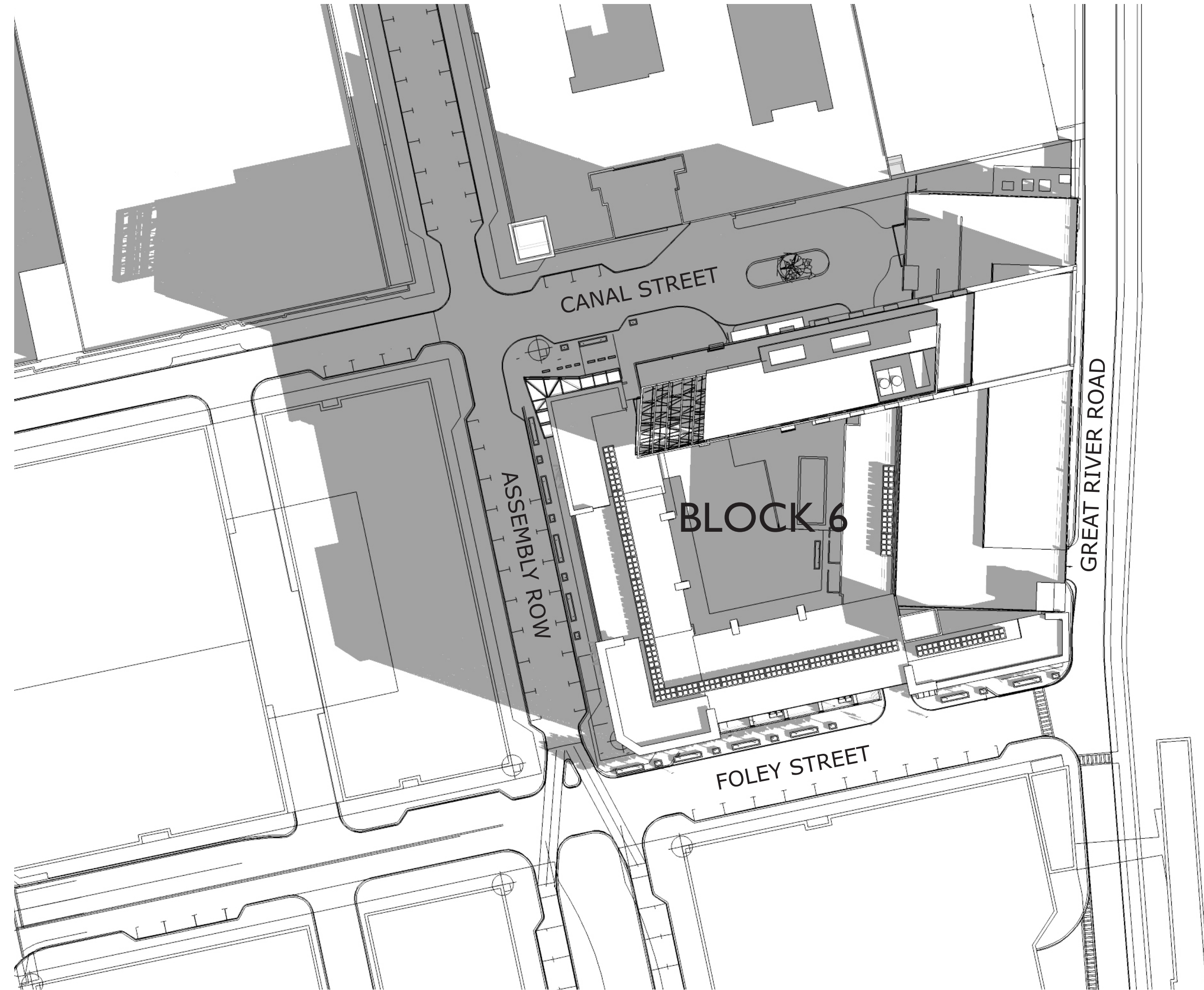
JUNE 21, 10 AM
