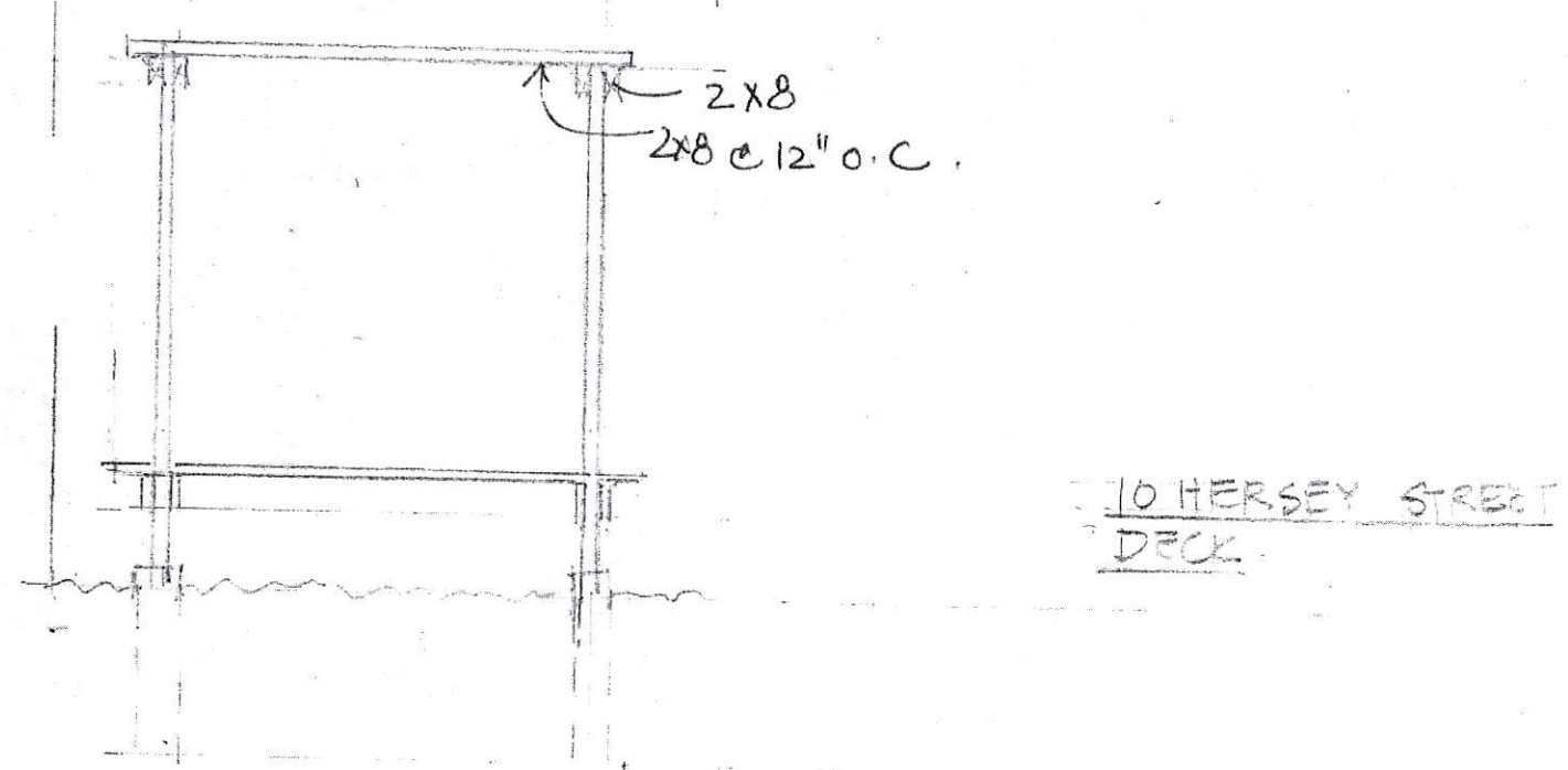
SECTION X-X
