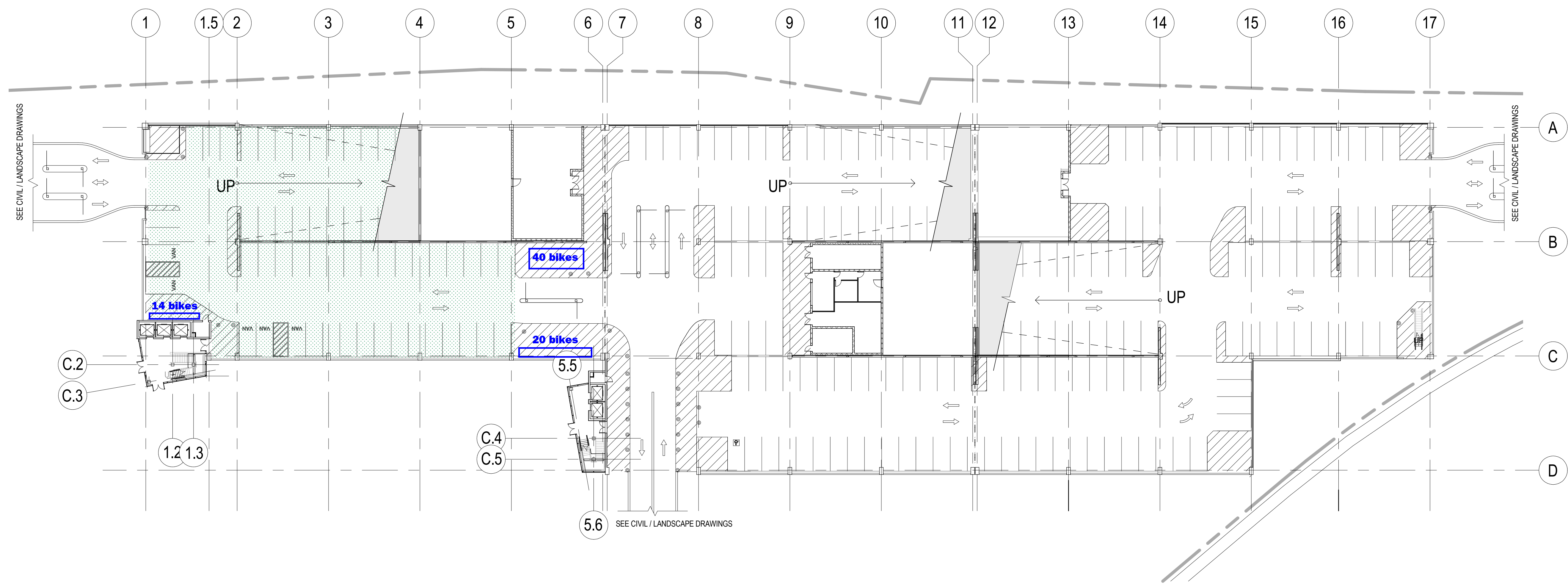
PARKING LEVEL 1
