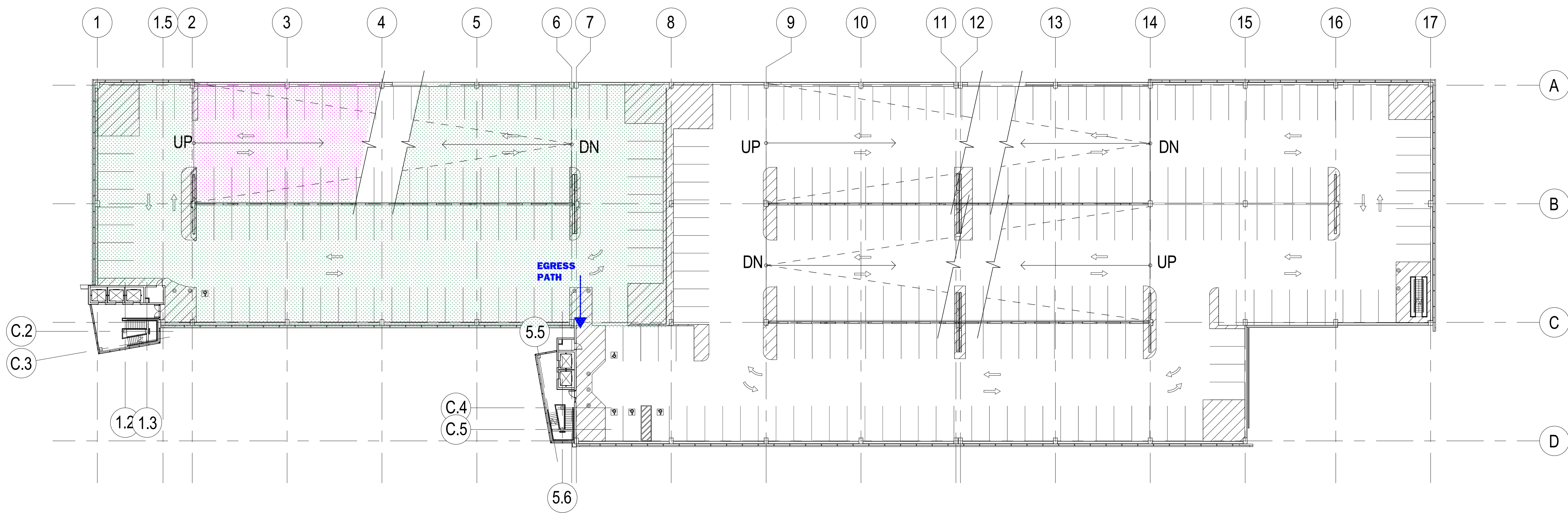
PARKING LEVEL 4
