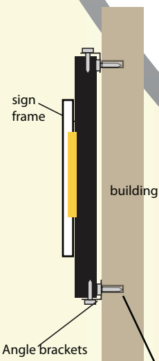
Lag bolt and shield anchor
