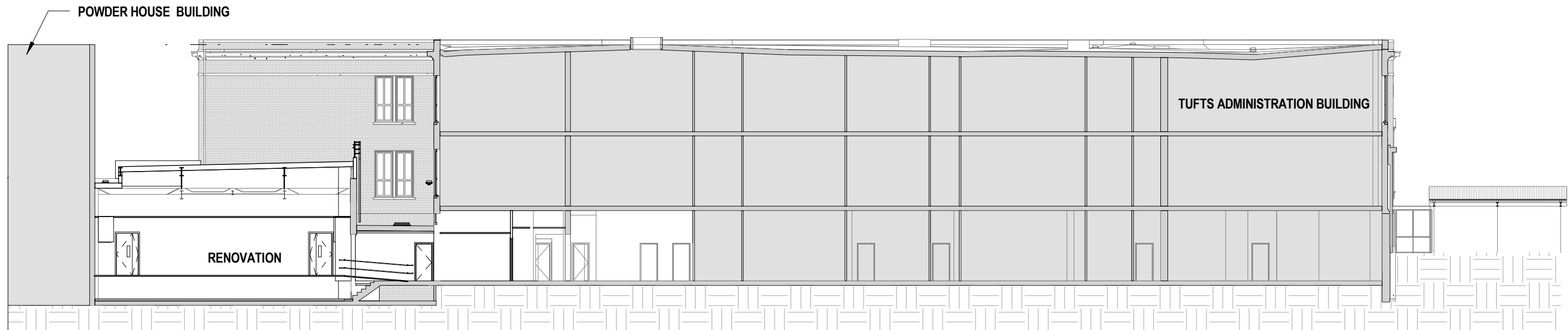
2 Section - Renovation 1" = 20'-0"
