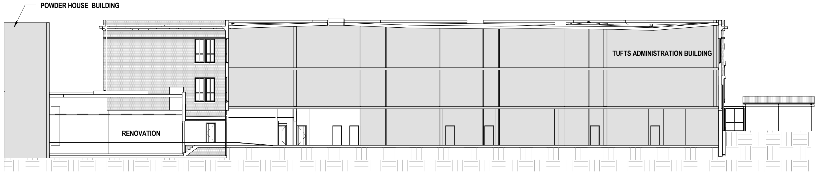
1 Section - Existing 1" = 20'-0"
