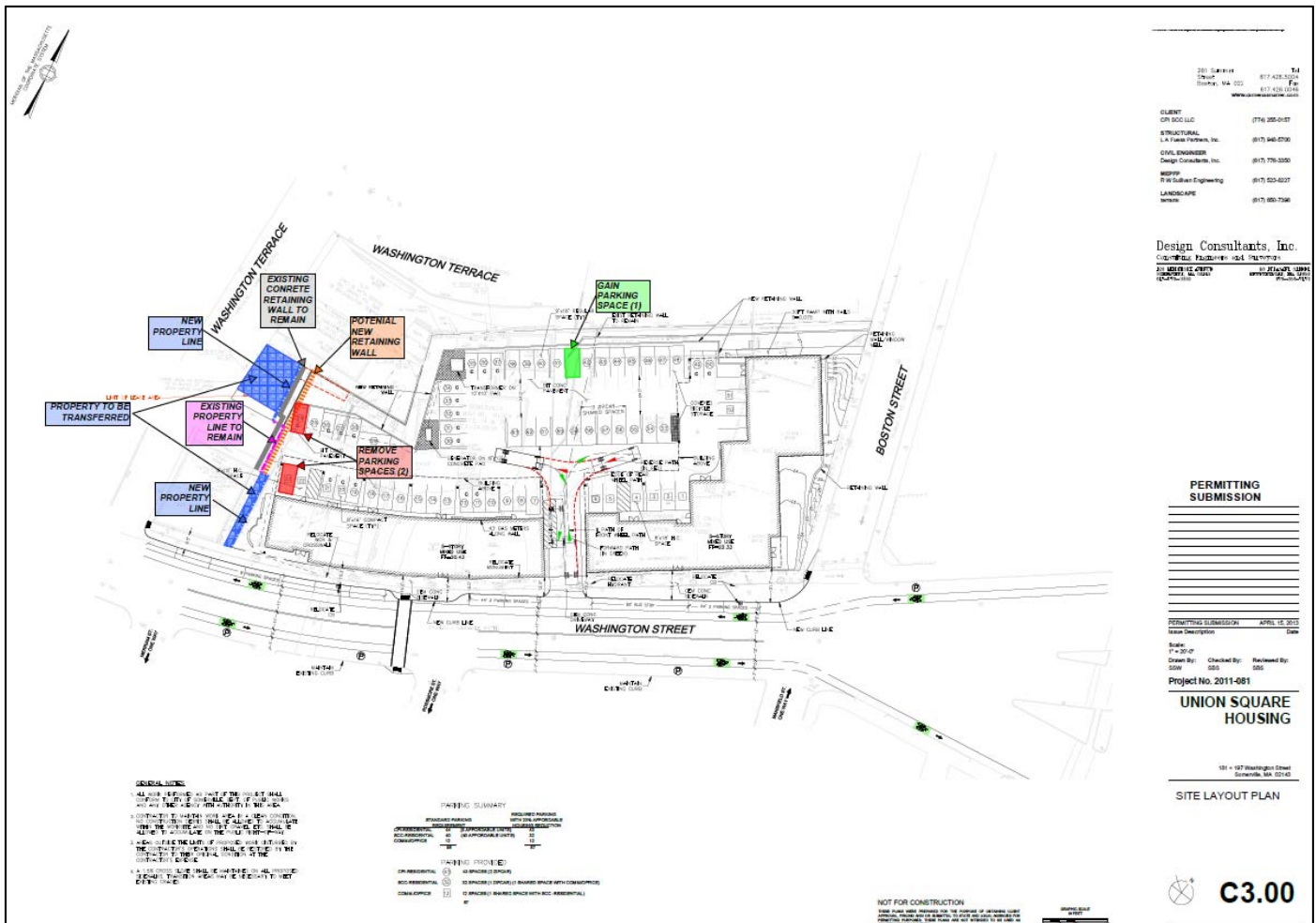
Figure 1: Site Plan
