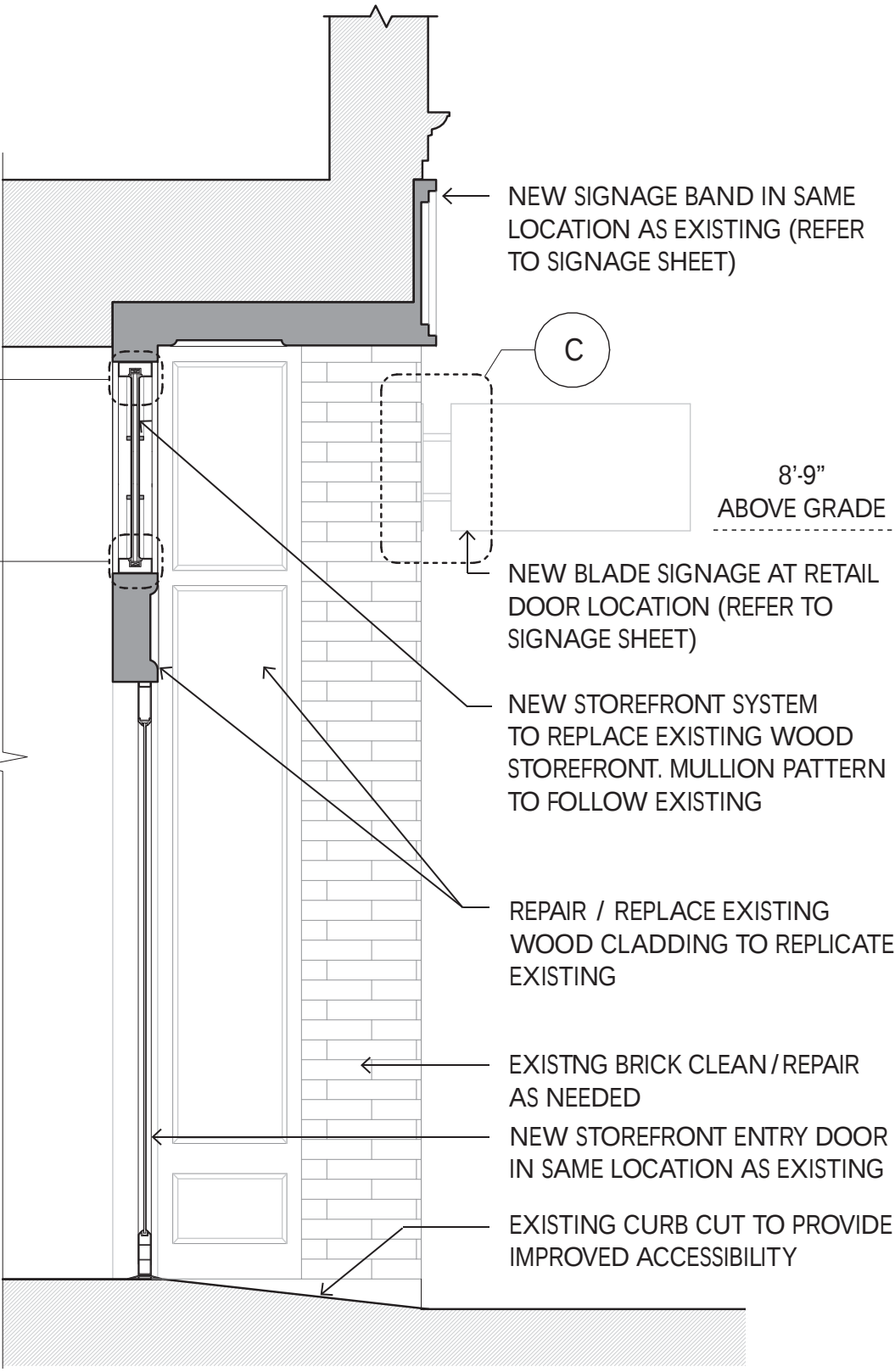
SECTION AT PROPOSED ENTRY
