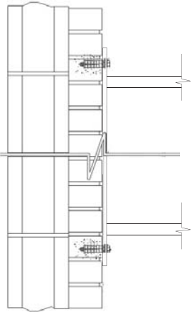
C. STOREFRONT SIGNAGE CONNECTION DETAIL
