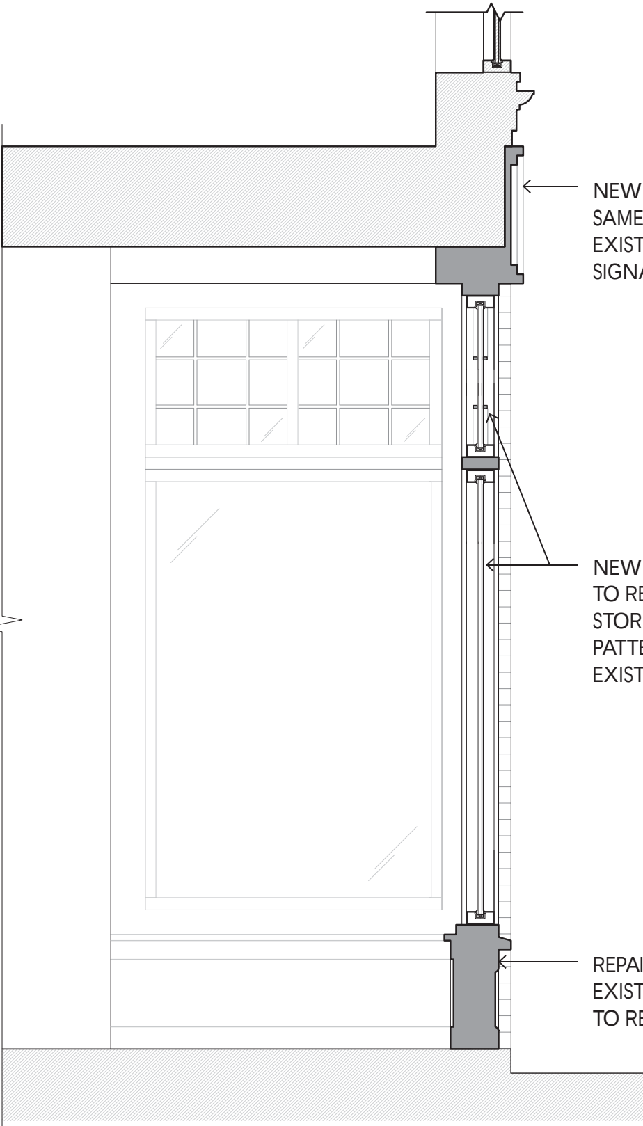
SECTION AT PROPOSED WINDOW
