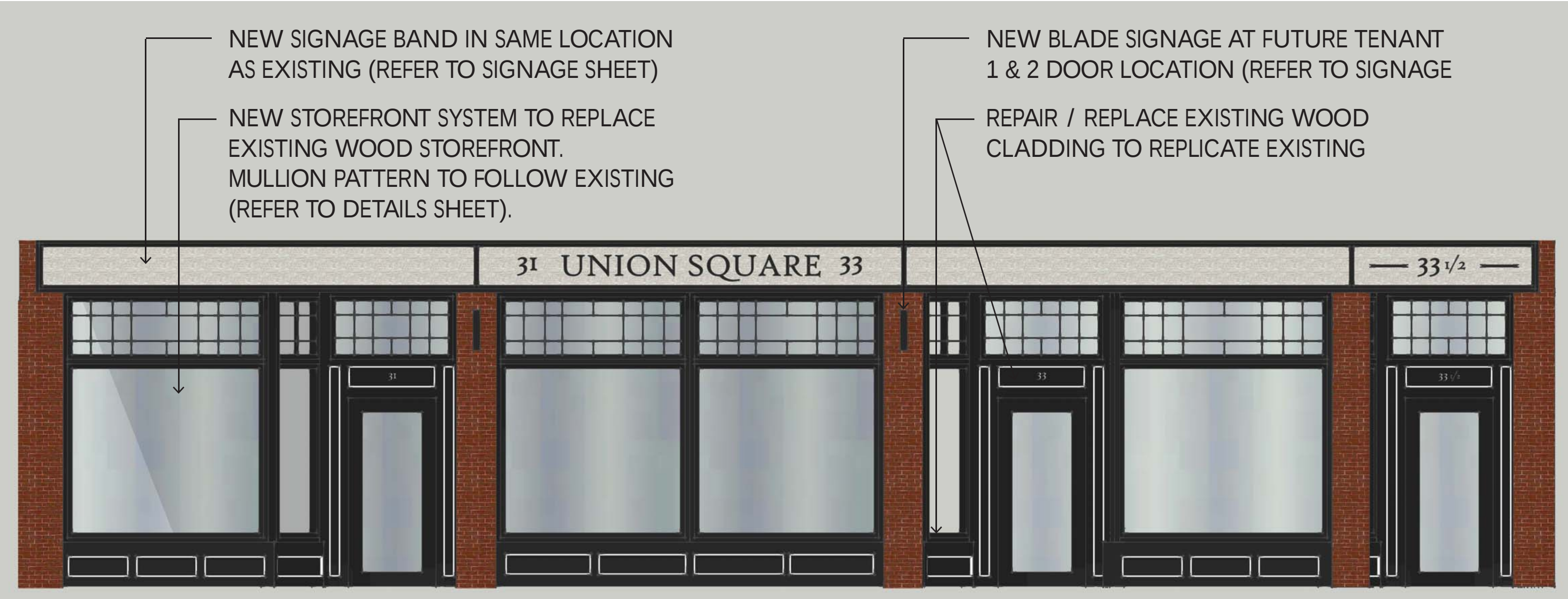
STOREFRONT ELEVATION
