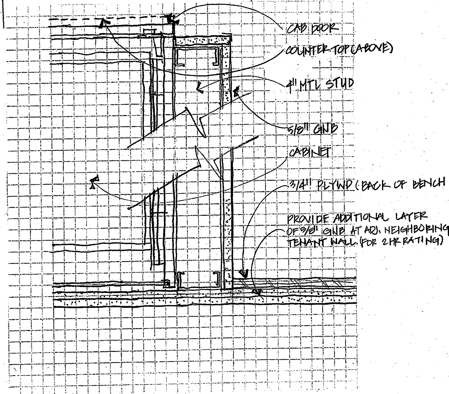
3. GNB CABINET INSTALLATION 3" = 1'-0"
